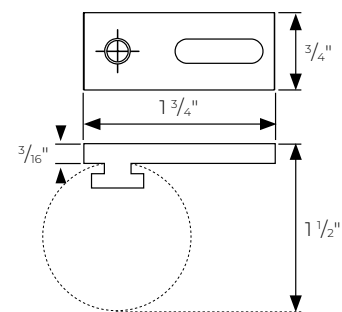
Low-Profile Ceiling Single PTHMT138406
