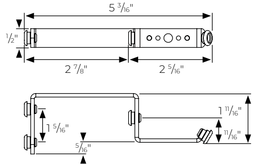
R-TEC Motorized Heavy Duty Traverse ONLY Ripplefold Butt Master Carrier Arm, One-Way Draw, Right or Left - RTMDTOB
